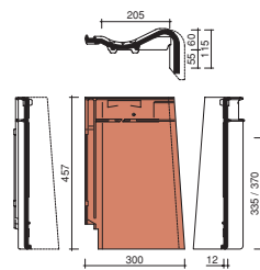
Madura Narvik cloaked verge tile right hand (2,7/m)
