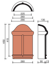
Tegelen 225mm interlocking half round begin hip tile
