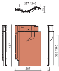
Madura Narvik ventilation tile with ceramic grid
