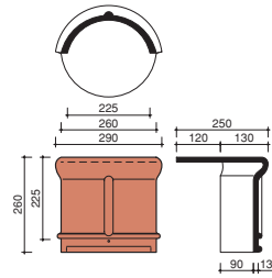
Tegelen 225mm interlocking half round starter ridge with end cap
