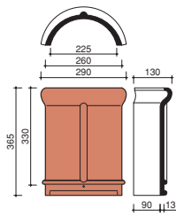
Tegelen 225mm interlocking half round ridge (3/m)
