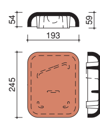
Tegelen cap for steam exhausting tile Ø 100 mm
