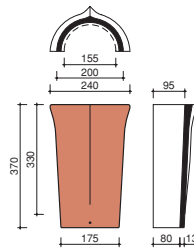
Tegelen tapered hip tile (3/m)
