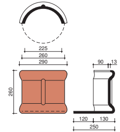
Tegelen 225mm interlocking half round end ridge with end cap
