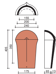
Tegelen begin tapered hip tile
