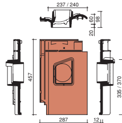
Madura Narvik steam exhausting tile Ø 100 mm
