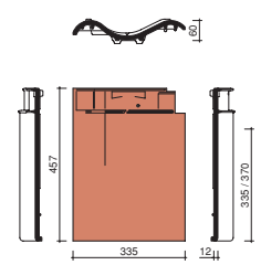
Madura Narvik Left hand verge/ Double roll tile (2,7/m)
