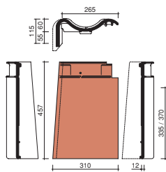
Madura Narvik cloaked verge tile left hand (2,7/m)
